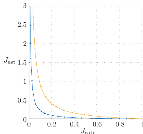
Figure 3: The trade-off between average communication rate J_{\text{rate}} and weighted average error cost J_{\text{est}} when using quadratic threshold policies for the example system. The upper curve shows the error costs achieved when a_t is IID Bernoulli with probability J_{\text{rate}} . The lower curve shows the error costs achieved using the proposed quadratic threshold.
