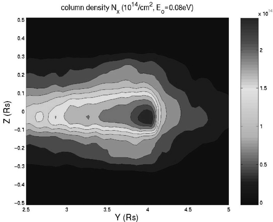
FIG. 2.—Monte Carlo model for the column density of gas in a neutral torus formed from an outgassing moon. The torus is seen edge-on. The horizontal and vertical axes are the distance from the planet in the orbital plane and perpendicular to the plane, respectively, in Saturn radii. The orbital radius for the moon is the same as that of Enceladus, 3.9R_s . The model parameters are S\tau = 10^{35} , v_e = 2 \text{ km s}^{-1} , and v_o = 12.6 \text{ km s}^{-1} . The ratio v_e/v_o determines the vertical and radial extents of the torus. (See text for details.)
