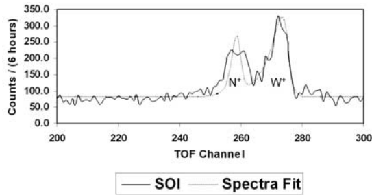
Figure 1. LEF spectrum for SOI orbit (day 182) from 18:00 to 24:00 UTC. The solid line shows ion counts corrected for fixed-pattern noise and integrated over 6 hours at 333 eV. The dotted line shows our model fit to the spectrum with the N^+ peak on the left and the water group ion ( W^+ ) peak on the right. The one sigma fractional uncertainties are \sim 1.5\% for both peaks with a chi-squared value of 3.8.
