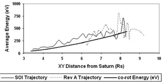
Figure 5. Average energy of ions entering N^+ (TOF channel 257) as a function of radial distance from Saturn along its equatorial plane for 6 hours of the SOI orbit (solid line) and 12 hours of Rev A (dotted line). The heavy solid line represents co-rotation energy.
