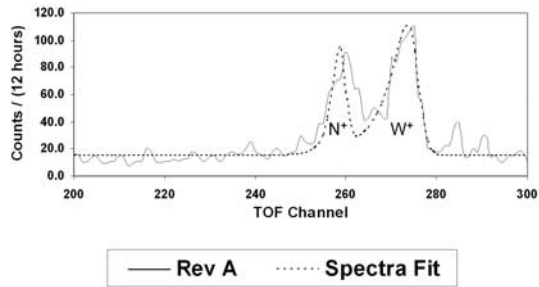
Figure 3. LEF spectrum for Rev A orbit (day 302) from 12:00 to 24:00 UTC. The solid line shows ion counts corrected for fixed-pattern noise and integrated over 12 hours at 333 eV. The dotted line shows our model fit to the spectrum with the N^+ peak on the left and the water group ion ( W^+ ) peak on the right. The one sigma fractional uncertainty for N^+ is \sim 7\% and 16\% for W^+ with a chi-squared value of 2.5.
