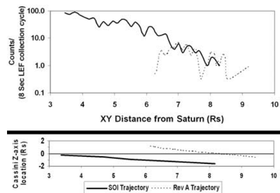
Figure 6. Ion counts (per 8 second LEF collection cycle) for detected N^+ as a function of radial distance from Saturn along its equatorial plane for 6 hours of the SOI orbit (solid line) and 12 hours of Rev A (dotted line). The lower portion shows Cassini's location normal to the orbital plane in Saturn Radii ( R_S ).
