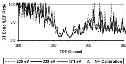
Figure 4. Ratio of ST "echo" peak ion counts to the associated LEF ion counts (TOF channels 200–350) collected during Rev A (12 hour integration) at three energy levels. The shaded triangle represents the ratio of the ST echo peak to the LEF peak derived from N^+ prototype calibration data.
