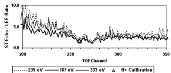
Figure 2. Ratio of ST "echo" peak ion counts to the associated LEF ion counts (TOF channels 200 to 350) integrated over the 6-hour SOI period at three energy levels. The shaded triangle represents the ST echo peak to LEF peak ratio derived from N^+ prototype calibration data.
