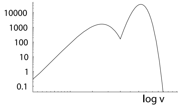
Figure 3. The appearance of a theoretical shell distribution in a count/velocity (energy) plot. The horizontal axis shows log speed, the vertical axis is counts in arbitrary units. The minimum in the middle part of the spectra is related to the drift velocity u , the two peaks around it to the shell radius w . The width is proportional to v_T . This plot is qualitatively similar to the structure of the energy spectra shown in Figure 2; see text for further discussion. For this plot u = 500 km/s, w = 200 km/s, and v_T = 100 km/s were chosen.
