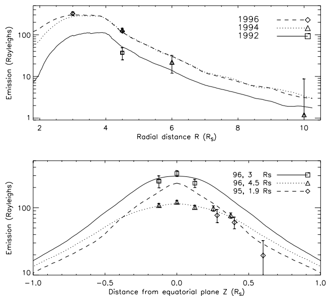
Figure 1. (a) Brightness profile of the OH cloud. Symbols represent inferred brightnesses from HST observations at the distances from Saturn as indicated, while lines represent modeled OH emission. (b) Same as (a) for vertical distance from the equatorial plane.
