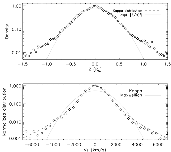
Figure 2. (a) The vertical density distribution of the OH cloud near Enceladus ( 3.5\text{--}4.5 R_S ). Diamonds represent model densities normalized to the density in the equatorial plane. The densities are poorly described by the commonly assumed Gaussian scale height (solid line): n(Z) = \exp(-(Z/H)^2) , where n is the density, H = 0.37 is the scale height, and Z is the distance from the equatorial plane. The 1-D Kappa distribution with kappa-index k = 1.9 provides a good fit (dashed line). (b) Same for the V_z component of the OH velocity distribution but with k = 2.0 .
