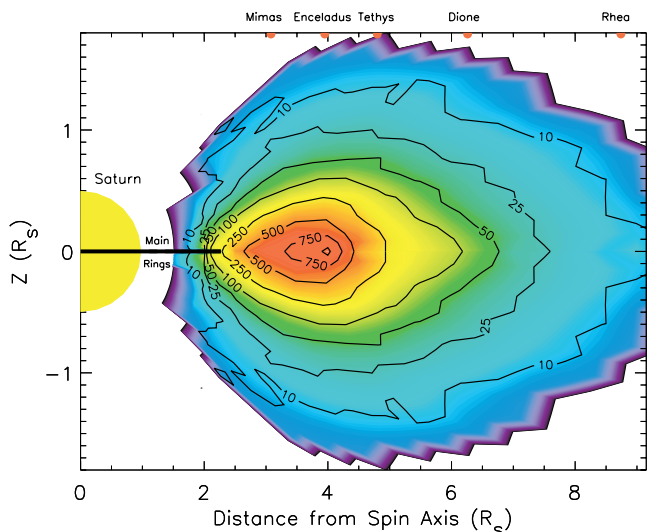
Figure 3. Cross section through Saturn's inner magnetosphere with OH density contours. Radial distances of major moons (red) are indicated on the X-axis, while the solid line represents the main rings. The sharp edges of the density contours (particularly the 500 and 750 \text{cm}^{-3} contours) between 4 and 5 R_S suggest the presence of a source close to Enceladus' orbit.
