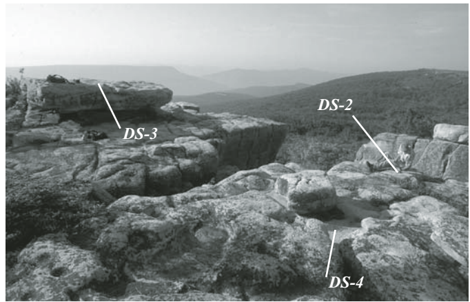
Figure 2. Photograph looking southeast over the edge of the Dolly Sods upland. Shown are sample collection locations for samples DS-2 (lower bedrock surface, note person for scale), DS-3 (upper bedrock surface with well-developed weathering pits), and DS-4 (residual quartz clasts).
