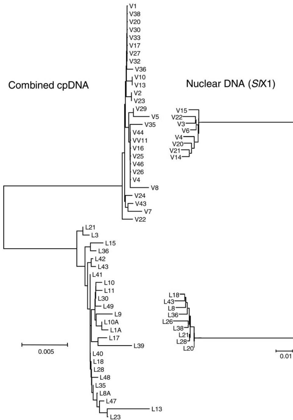
Fig. 1. Neighbor-joining trees for the chloroplast data and the nuclear gene, SIX1 , based on Jukes–Cantor distances. Chloroplast sequence diversity in S. vulgaris is reduced below neutral expectations as evidenced by the short branch lengths within the S. vulgaris clade, compared with S. latifolia . No difference in sequence diversity is seen between the two species at the nuclear gene, after correcting for X-linkage of SIX1 in S. latifolia . Note that the scale differs between the two neighbor-joining trees. VLG = samples of S. vulgaris ; LAT = samples of S. latifolia .
