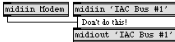
This patch will create a feedback loop of MIDI data
